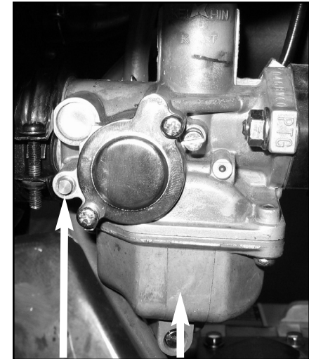
Air Screw
